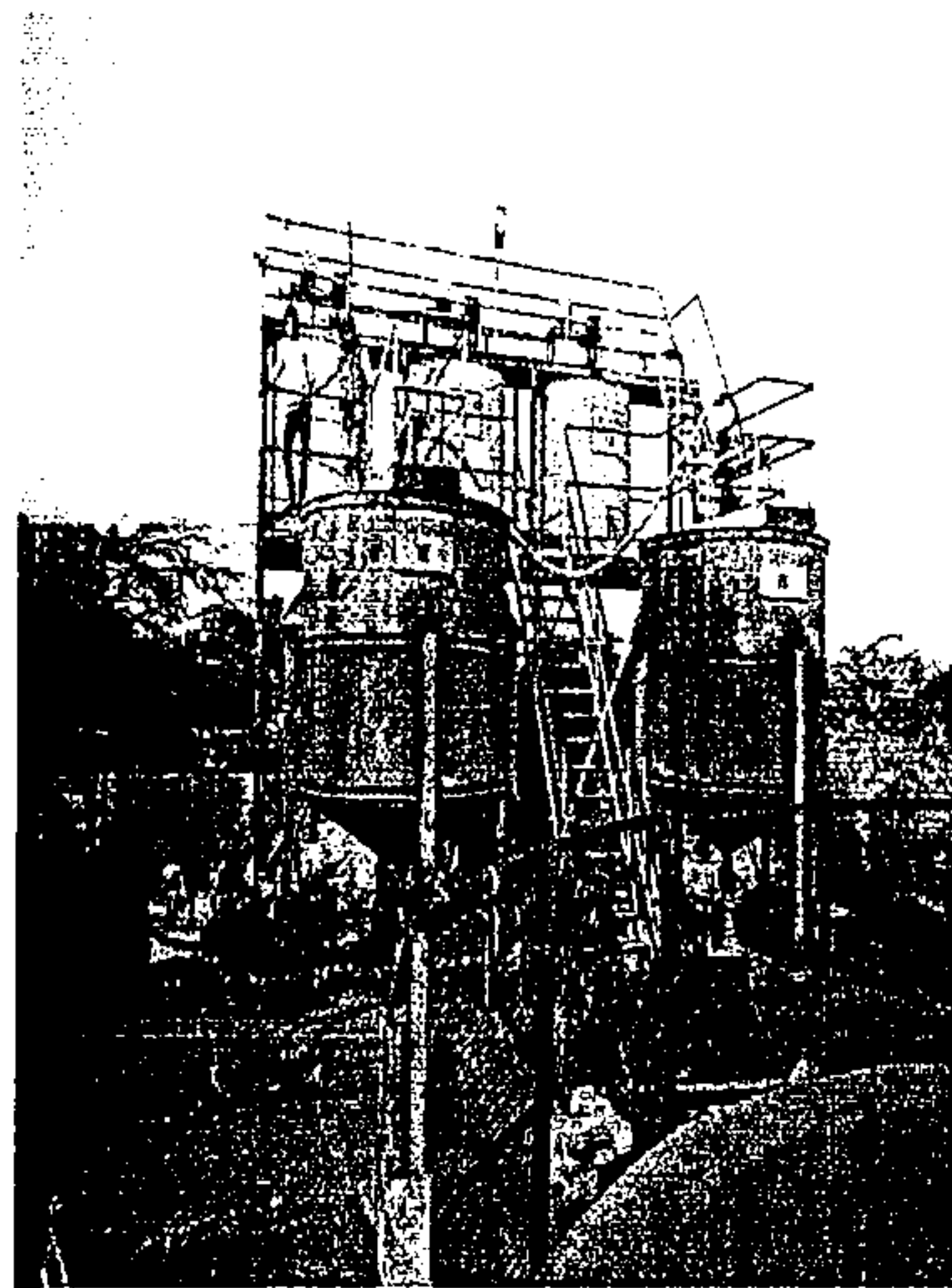
View of the separate Acid treatment plant
