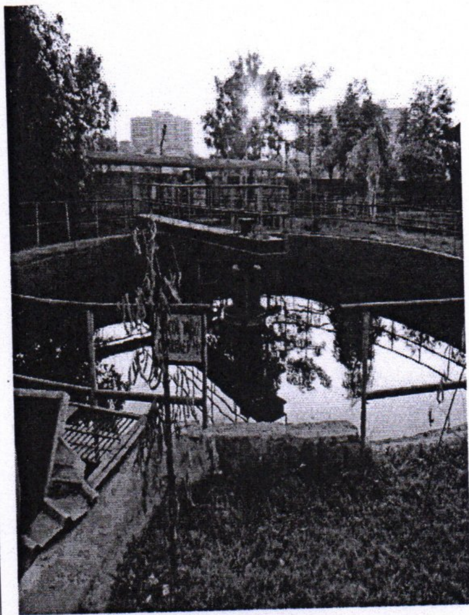
Secondary clarifier I & II
